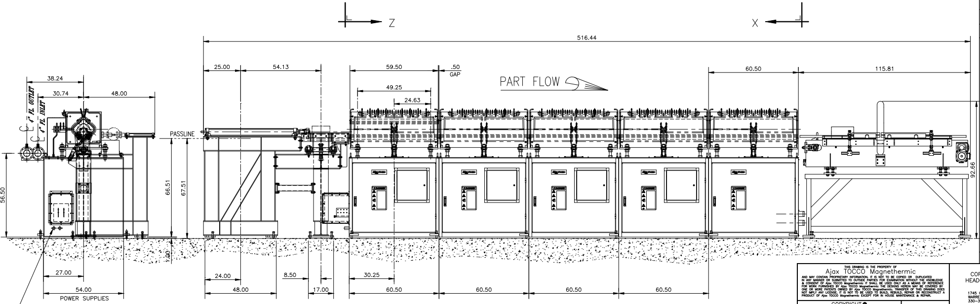
ELEVATION VIEW
