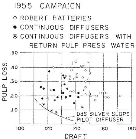
Figure 6.—Draft and pulp loss campaign results—American factories.
