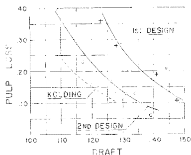
Figure 3.—Draft and pulp loss—first trial runs.
