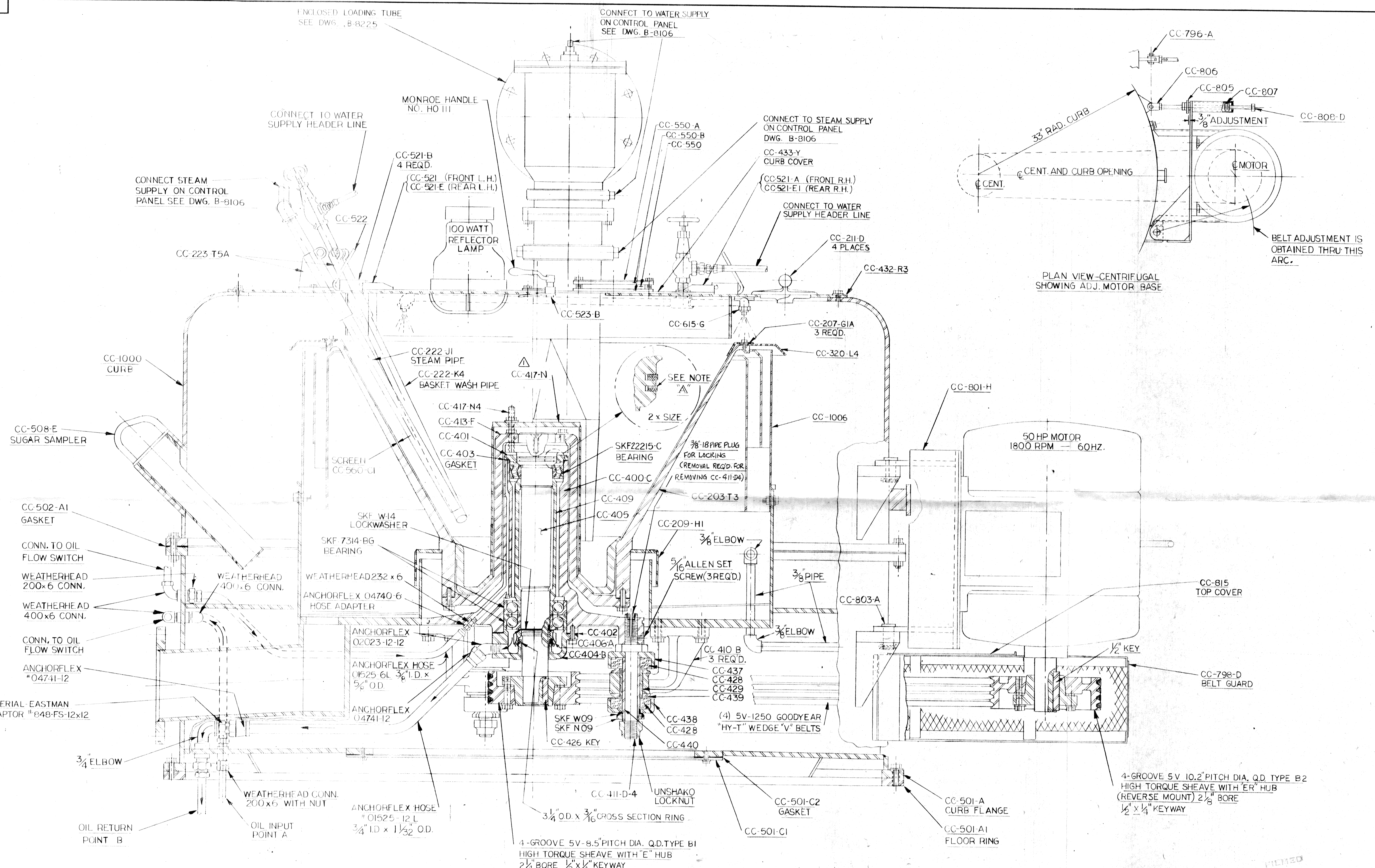
TYPICAL SECTION
