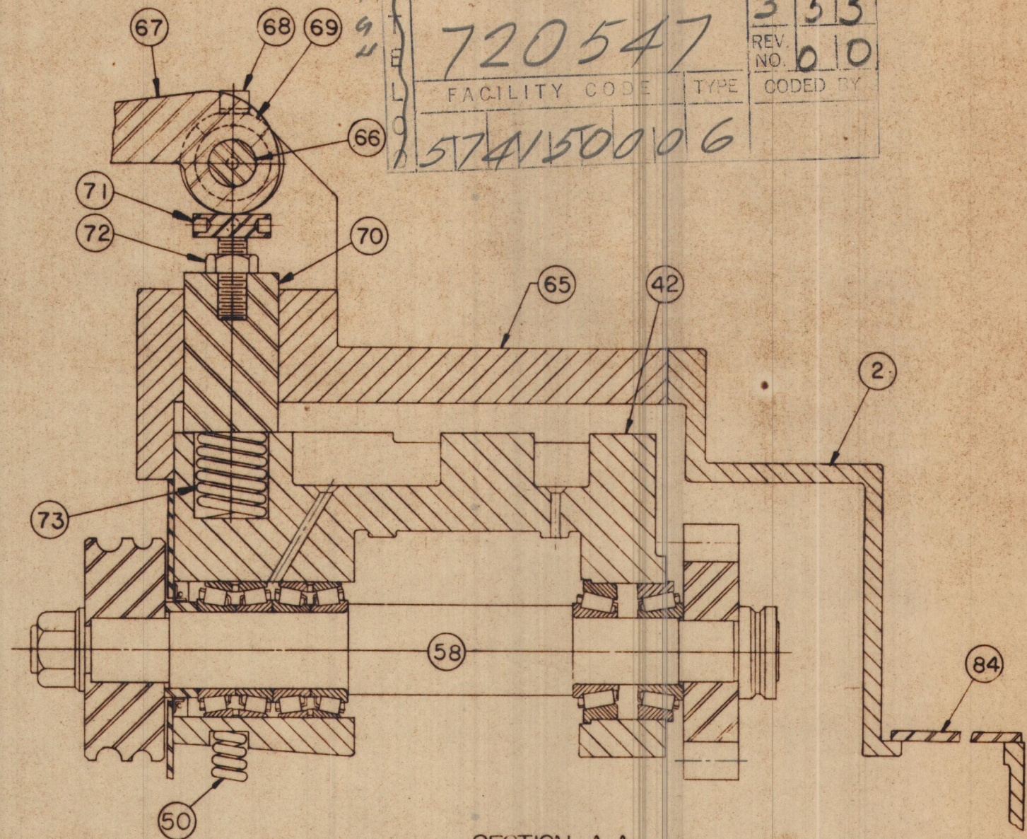
SECTION-A-A REAR HOUSING FEED ASSEMBLY
