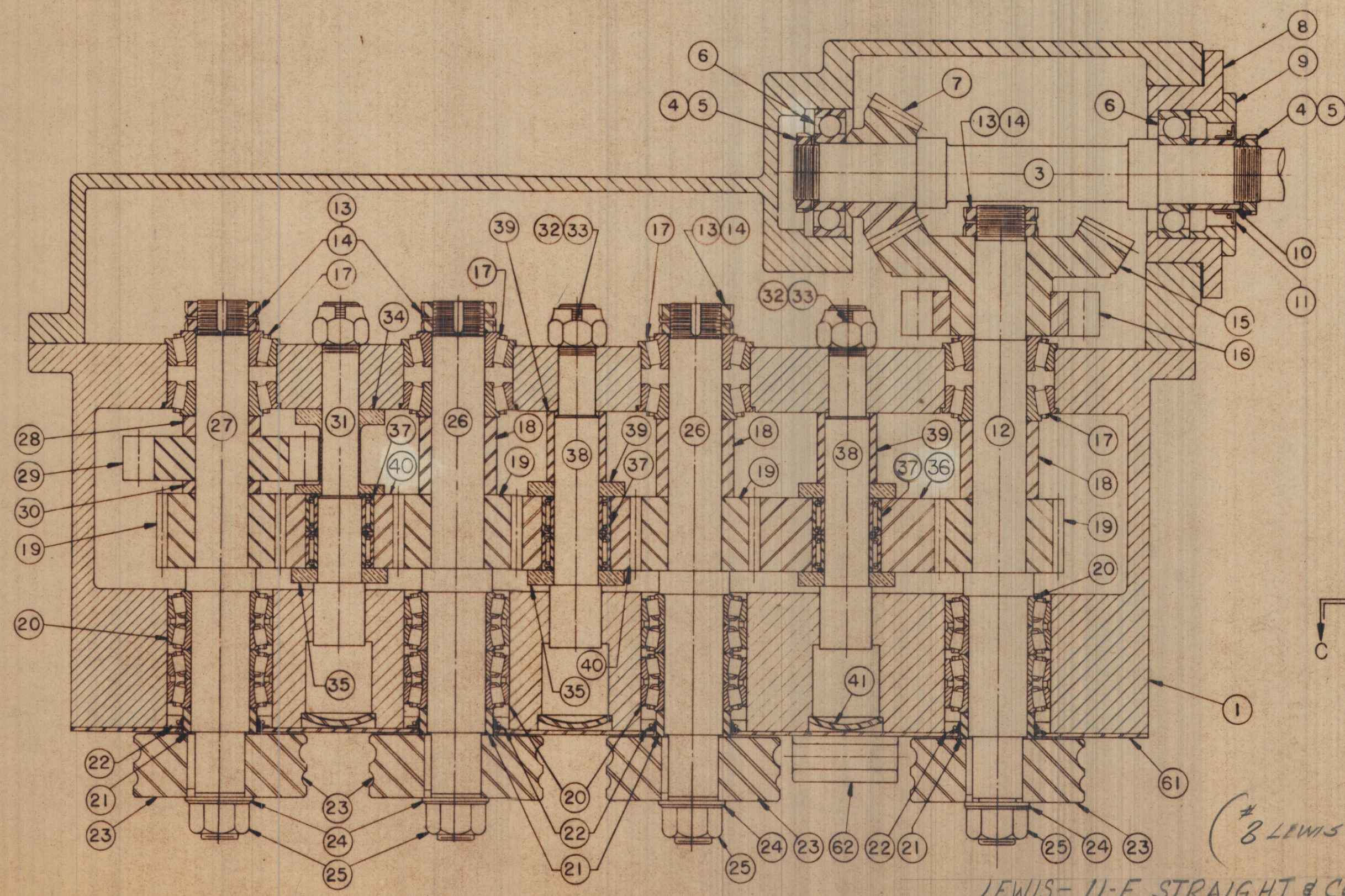
SECTION-CC REAR HOUSING LOWER FEED AND STRAIGHTENER ASSEMBLY
