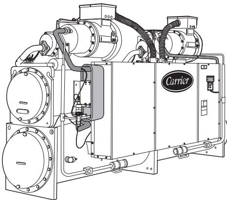
TWIN-SCREW COMPRESSOR DESIGN
